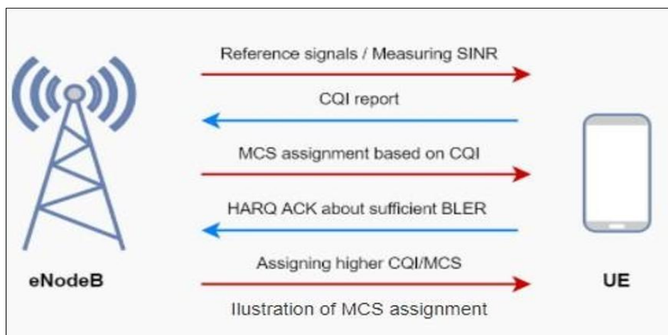
Figure 1: CQI (Channel Quality Indication)
