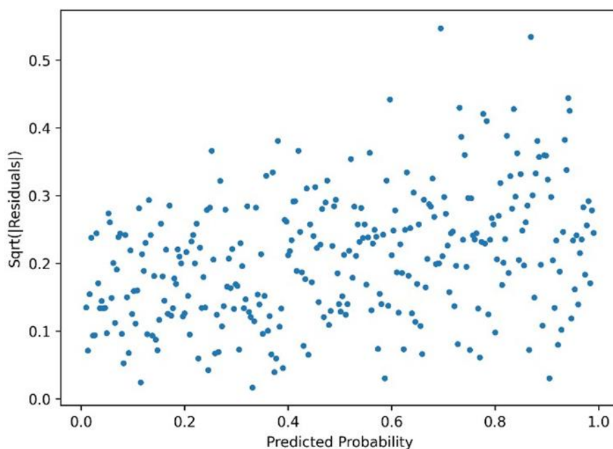
Figure 11. Homoscedasticity Plot
