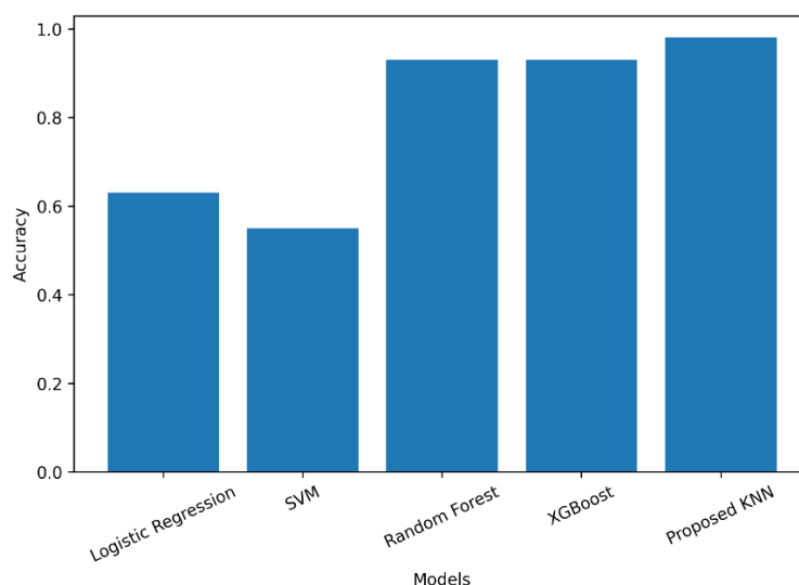
Figure 7. Overall Model Comparison Graph
