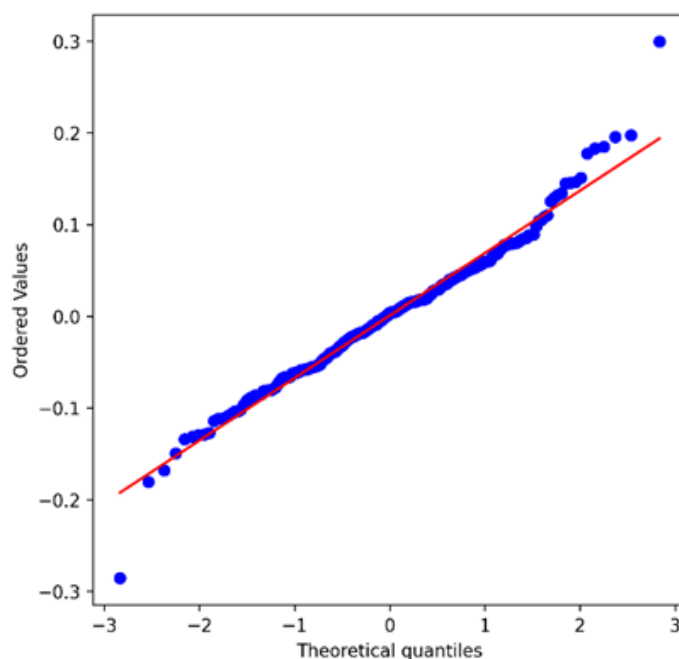
Figure 9. QQ Plot
