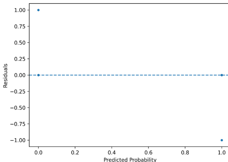
Figure 8. Residual Plot
